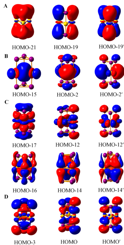
Figure 2. Plots of some key occupied MOs of [\text{Sb}_3\text{Au}_3\text{Sb}_3]^{3-} cluster, generated by GaussView (Sb: purple, Au: yellow). 38 (A) Sb → Au donation: HOMO-21 and HOMO-19/HOMO-19'. (B) Au 6s based MOs: HOMO-15 and HOMO-2/HOMO-2'. The latter two are responsible for Sb → Au donation of 3 electrons. (C) Au → Sb back-donation: HOMO-17, HOMO-12/HOMO-12', HOMO-16, and HOMO-14/HOMO-14'. (D) Globally delocalized three-center three-electron (3c-3e) bonds in the two cyclo -Sb 3 : HOMO-3 and HOMO/HOMO'. All these 15 MOs (except HOMO-15) collectively contribute to Au–Sb bonding in [\text{Sb}_3\text{Au}_3\text{Sb}_3]^{3-} .
